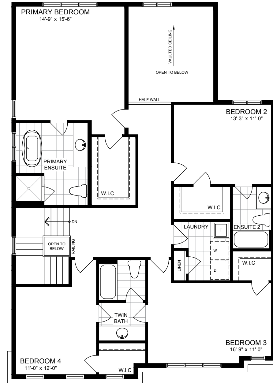
SECOND FLOOR STYLE A
