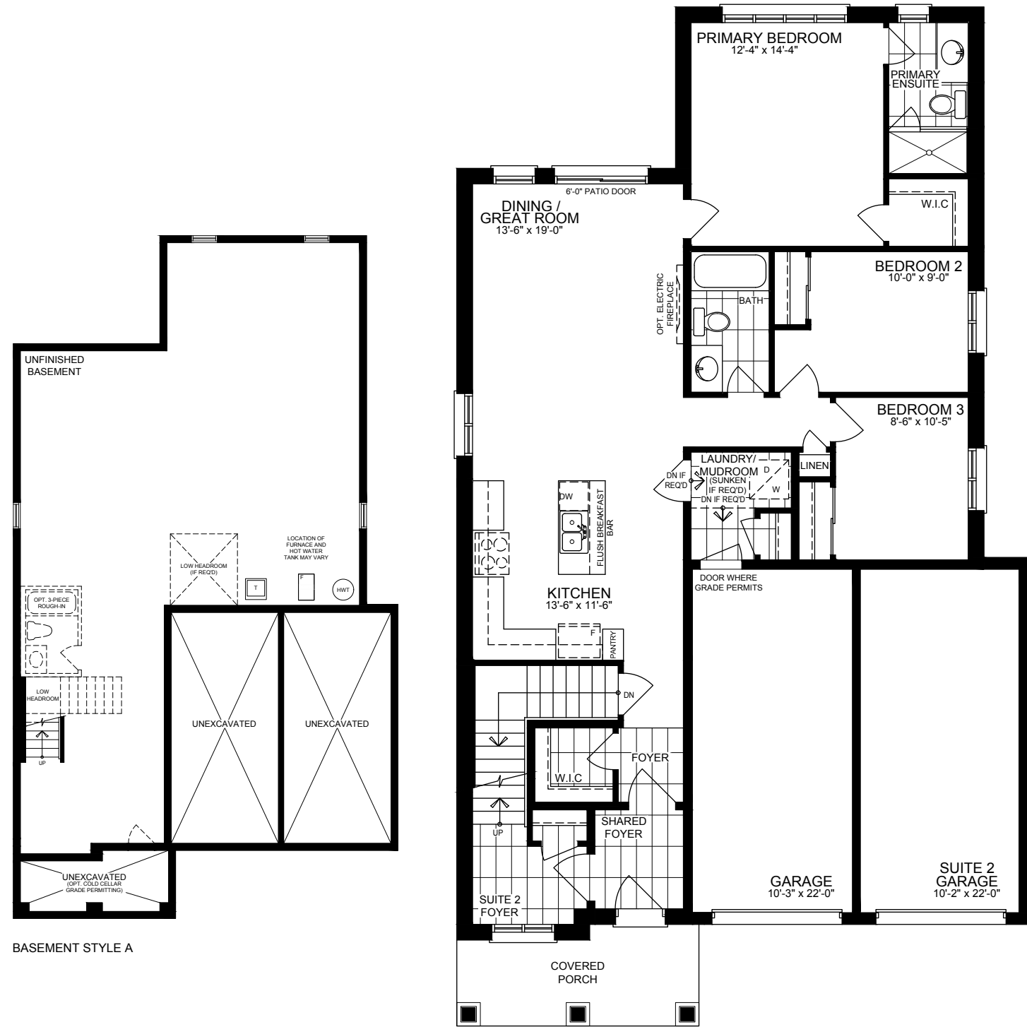
GROUND FLOOR STYLE A
