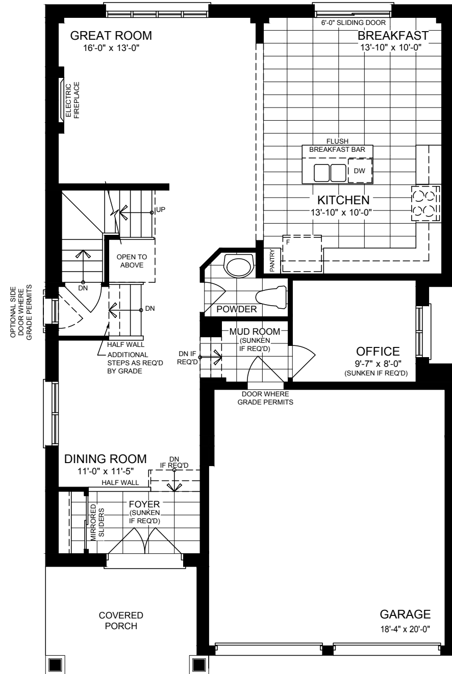
GROUND FLOOR STYLE A
