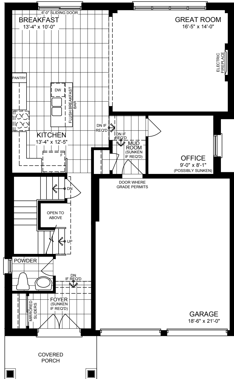
GROUND FLOOR STYLE A
