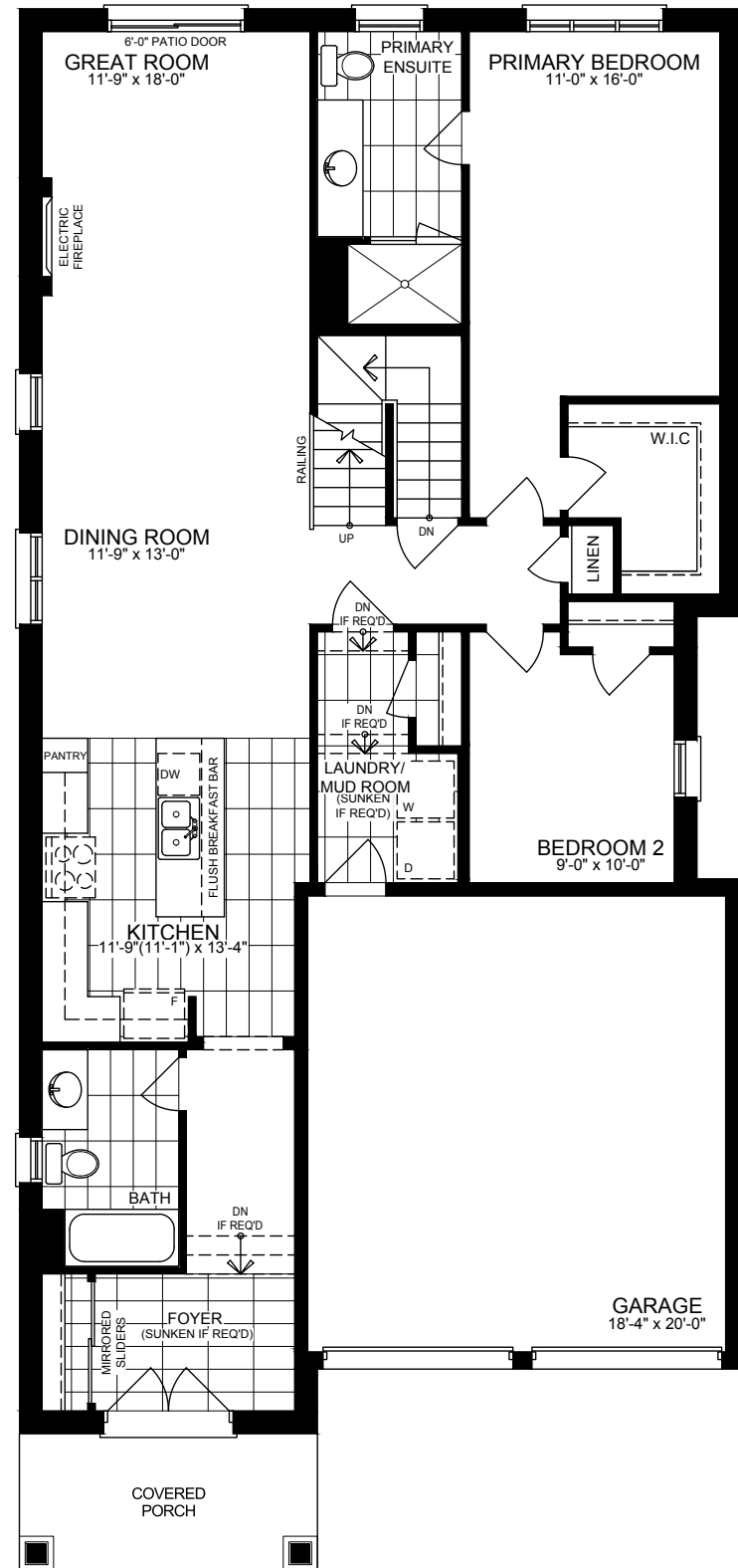
GROUND FLOOR STYLE A
