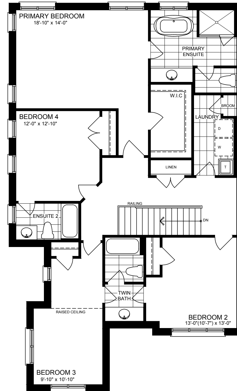
SECOND FLOOR STYLE B
