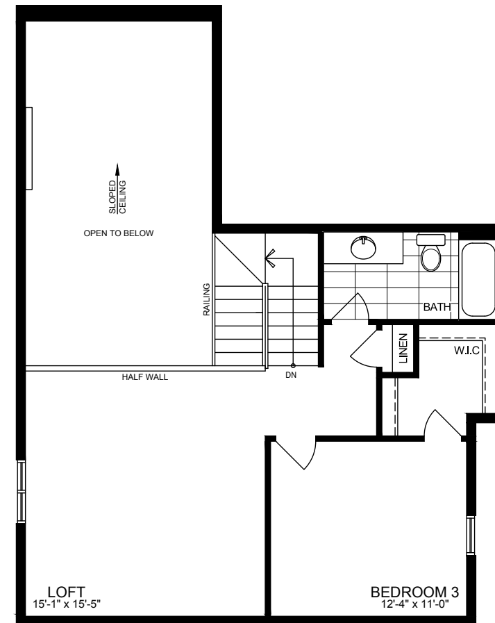
LOFT FLOOR STYLE A
