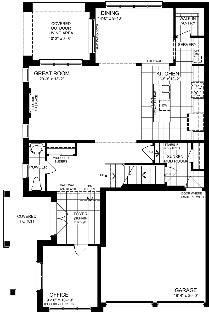
GROUND FLOOR STYLE B
