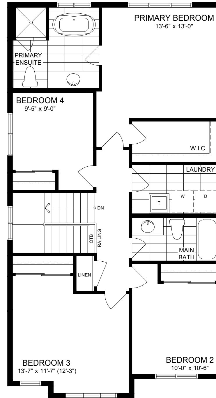
SECOND FLOOR STYLE A
