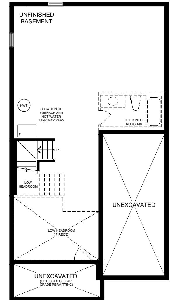
BASEMENT STYLE A
