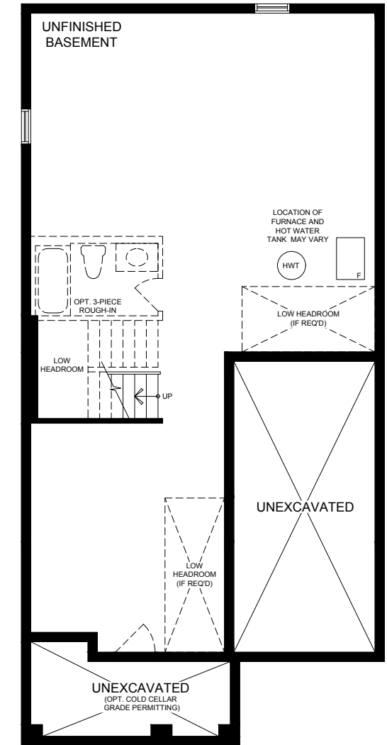
BASEMENT STYLE A
