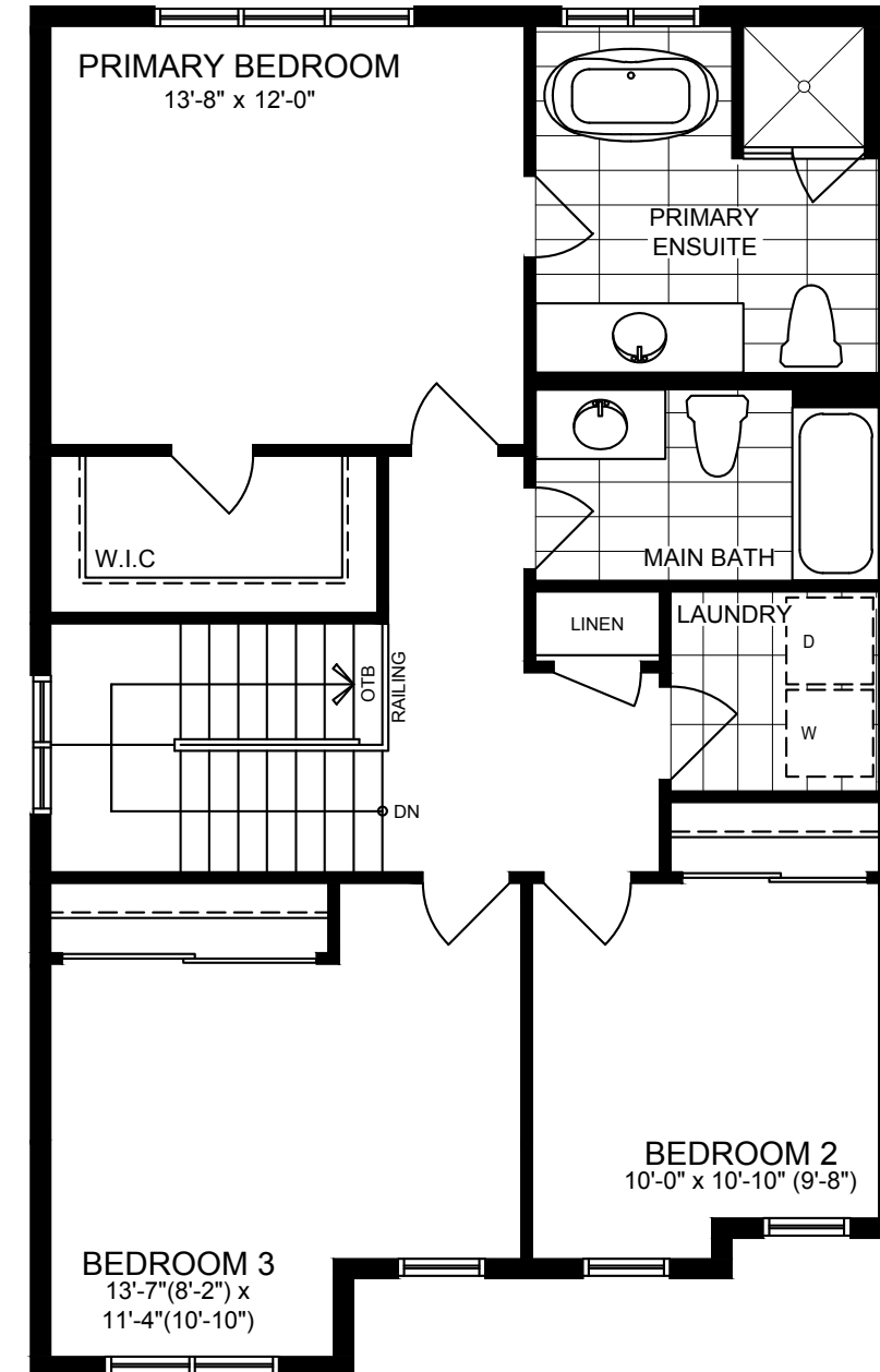
SECOND FLOOR STYLE A
