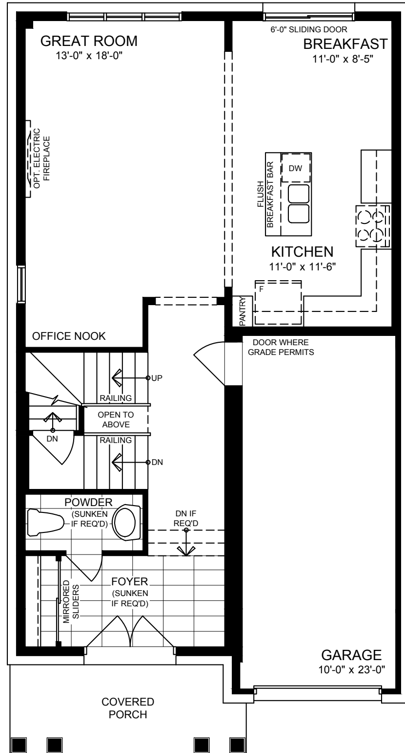
GROUND FLOOR STYLE A
