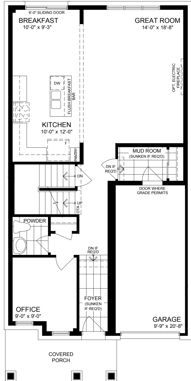
GROUND FLOOR STYLE A
