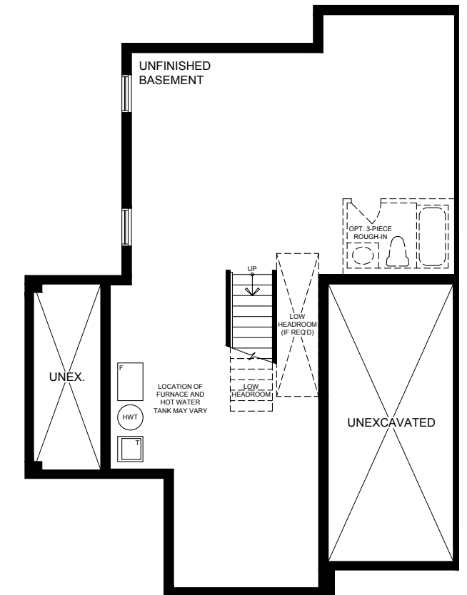
BASEMENT STYLE A
