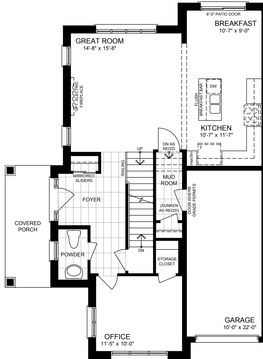
GROUND FLOOR STYLE A
